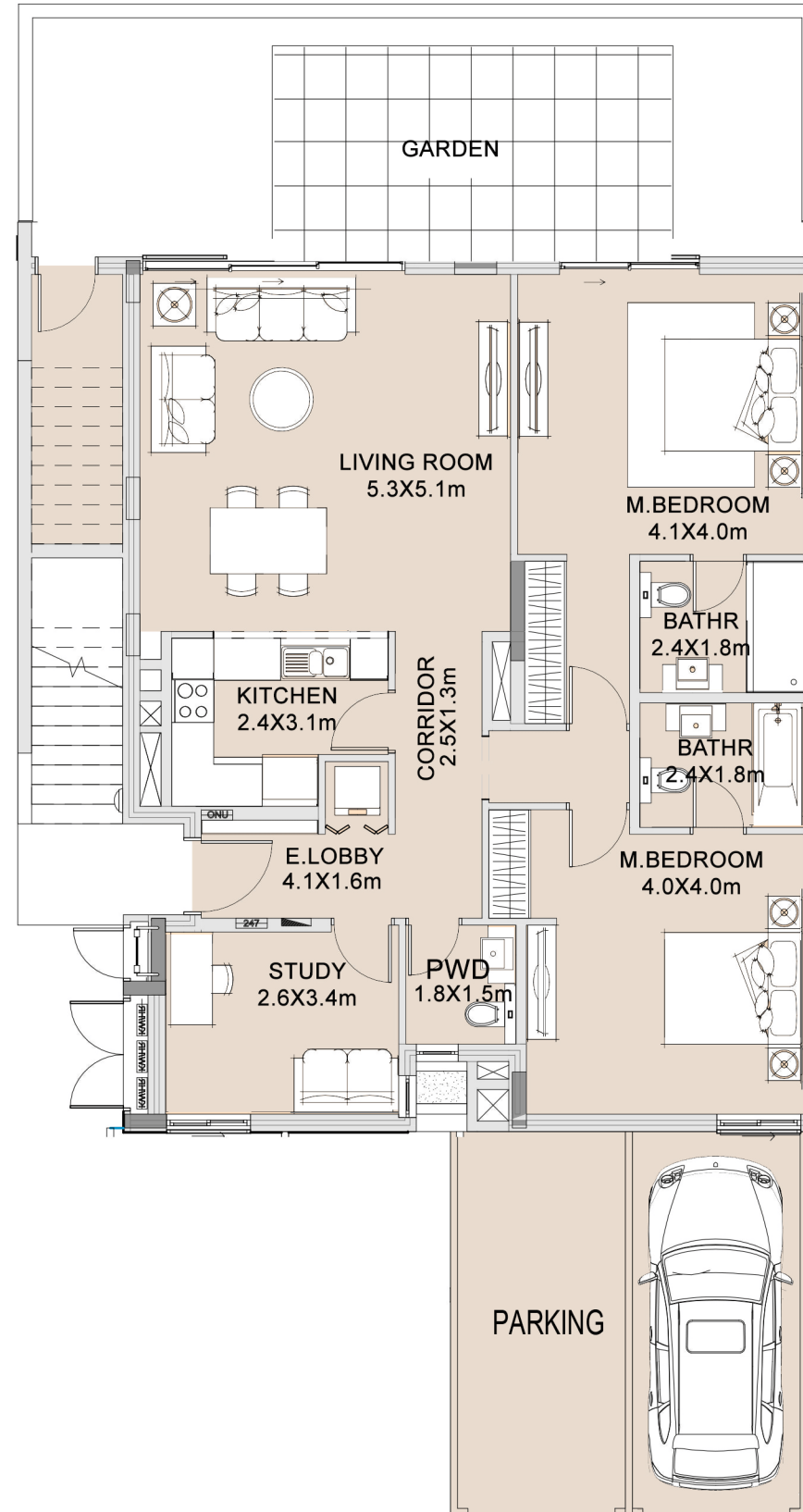
A-1-2B | Ground Level 1:100
