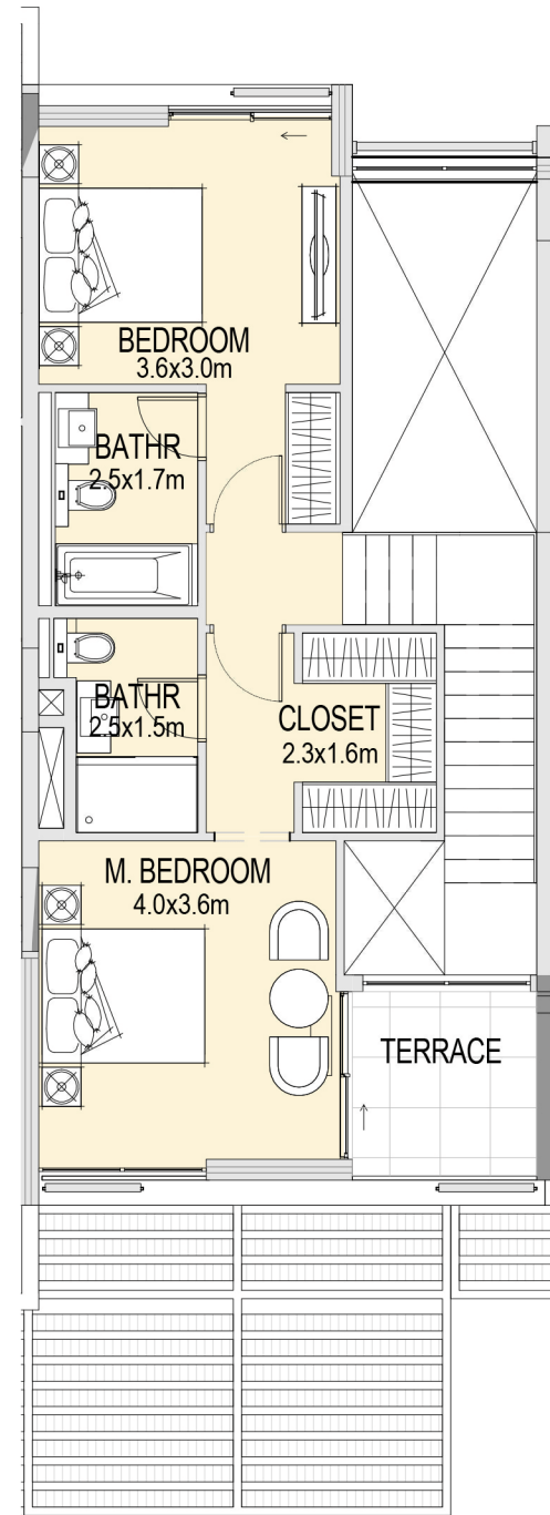
B-2-2B | Unit 2- Level 1 1:100
