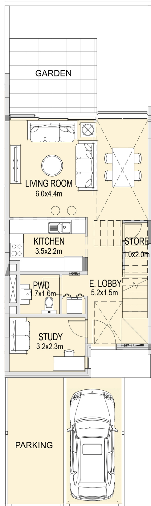
B-2-2B | Ground Level 1:100
