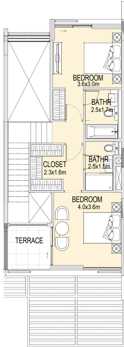
B-3-2B | Level 1 1:100
